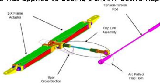
Figure 3 Straub-Kennedy Double X-Frame
