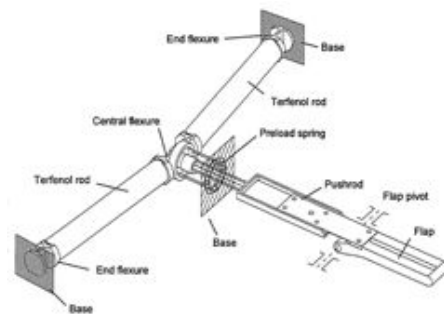
Figure 1 Bushko-Fenn V-stacks (magnetostrictive)
