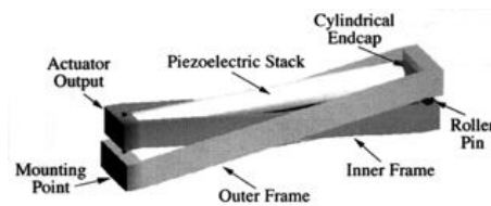
Figure 2 Precht-Hall X-Frame
