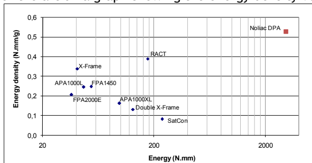
Figure 12 Energy density comparison
