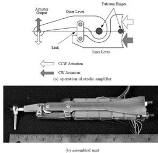
Figure 4 Lee-Chopra Differential stacks with L-L amplification
