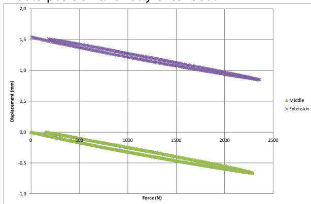
Figure 11 "Diamond frame" prototype force-displacement diagram
